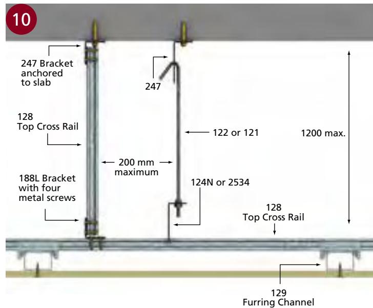
■ DOWNSTRUT DETAIL
