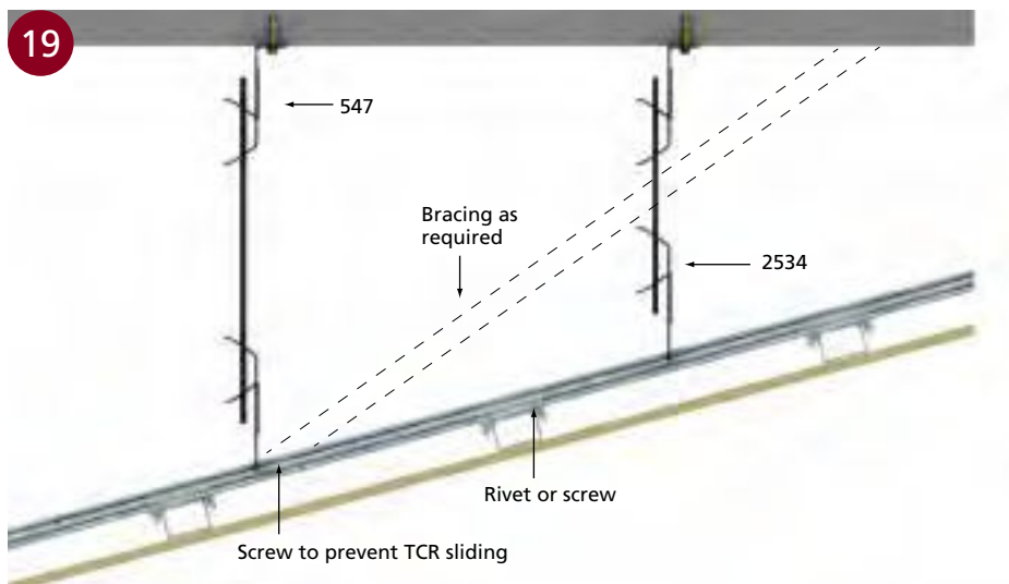
■ FOR RAKING AND CURVED CEILINGS
