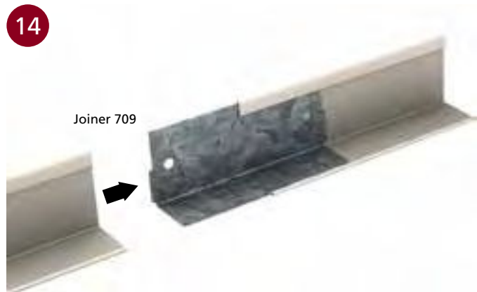
■ BULKHEAD DETAILS
