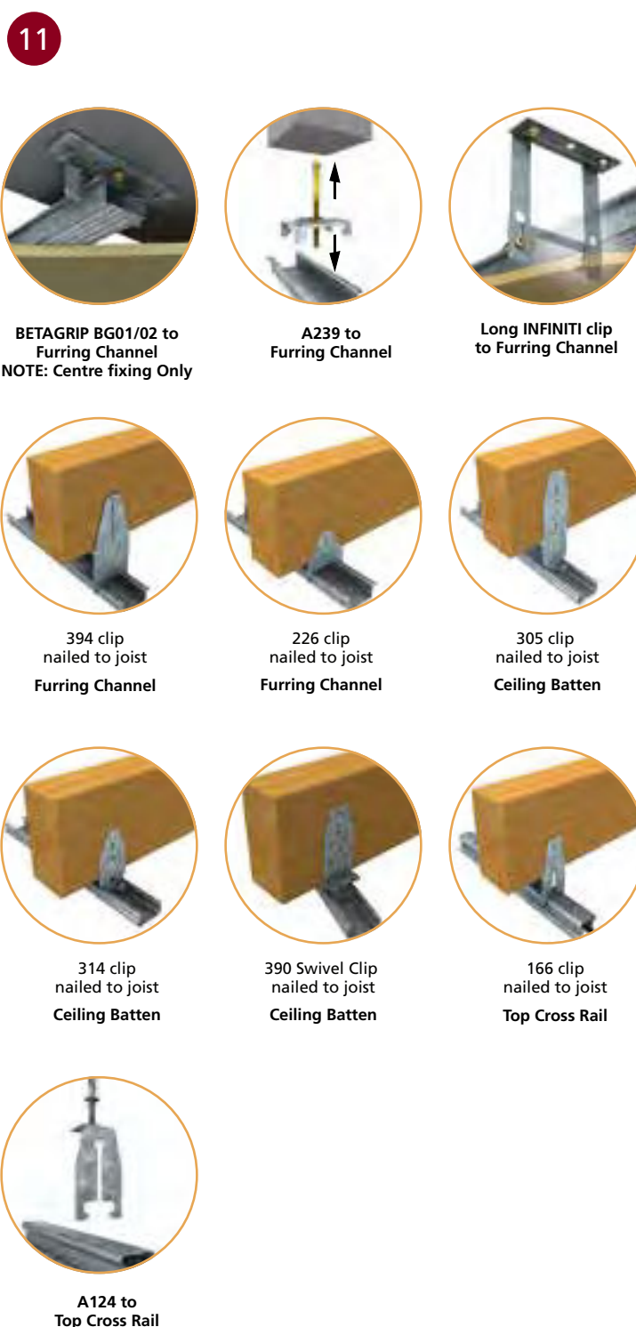
■ DIRECT FIXING CLIPS
