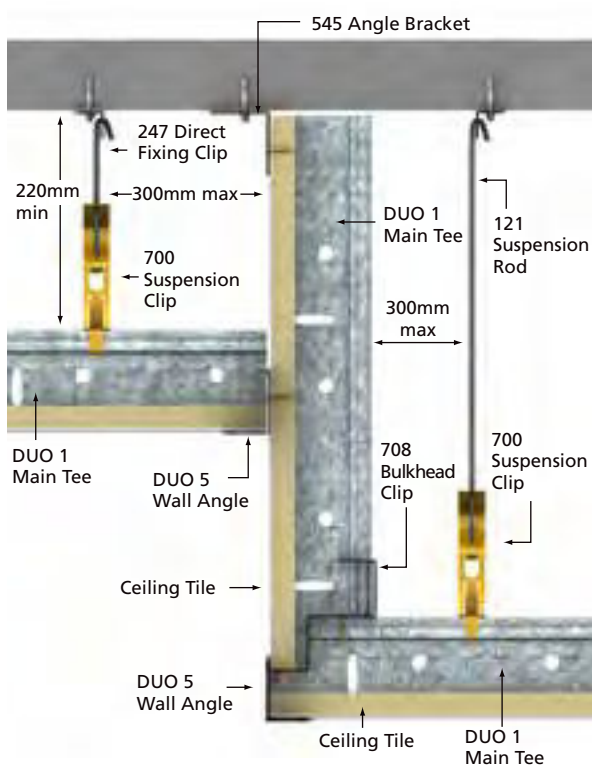
■ SQUARELINE BULKHEAD DETAIL (Vertical Exposed Grid)
