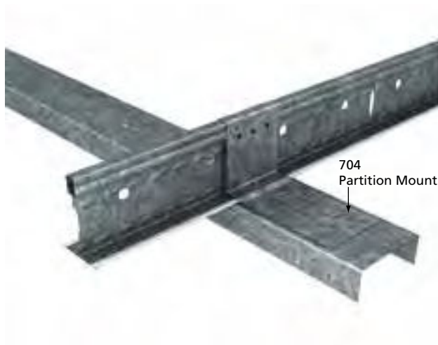
■ PARTITION MOUNTING DETAILS
