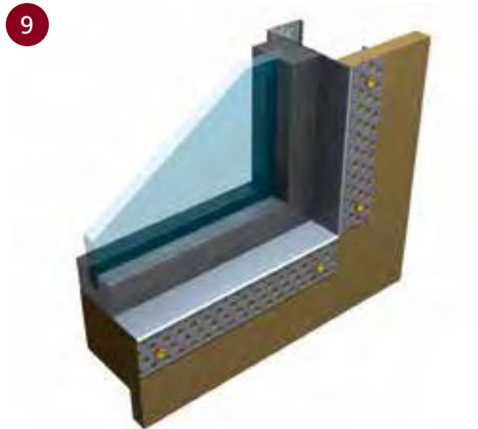
■ REVEAL BEAD INSTALLATION
